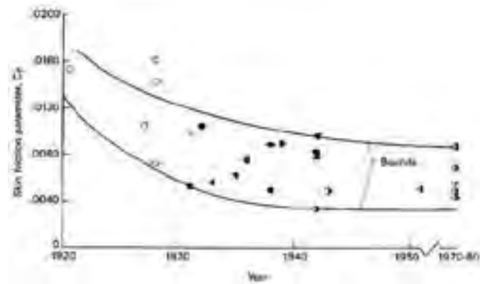
Figure 7.8 - Trends in skin friction Parameter C_F {ptr: line over C} of propeller-driven aircraft. [ref. 90].
