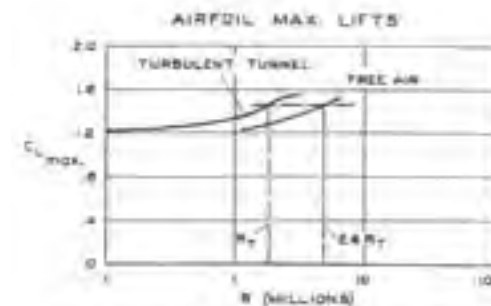
Fig. 6.—Airfoil Maximum Lift as Affected by Tunnel Turbulence
