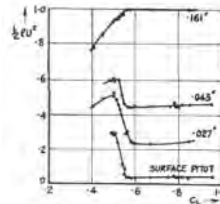
Fig. 5. Typical observations of total pressure in the transition region. These observations are from the five pitot tubes illustrated in Fig. 3, which were mounted on the upper surface of the wing of thickness ratio 0.18 at 0.37 chords from the leading edge. The numbers written on each curve show the distance of the orifice of the air shaped orifice from the wing surface. Ordinates represent the total pressure registered by the tubes and abscissae the lift coefficient of the whole aeroplane. As lift coefficient increased the transition point moved backwards on the wing past the orifices of the tubes.
