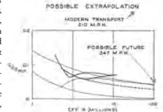
Fig. 12 - Possible Extrapolation of Tunnel Test Data into the Higher Full-Scale Range of the Reynolds Number
