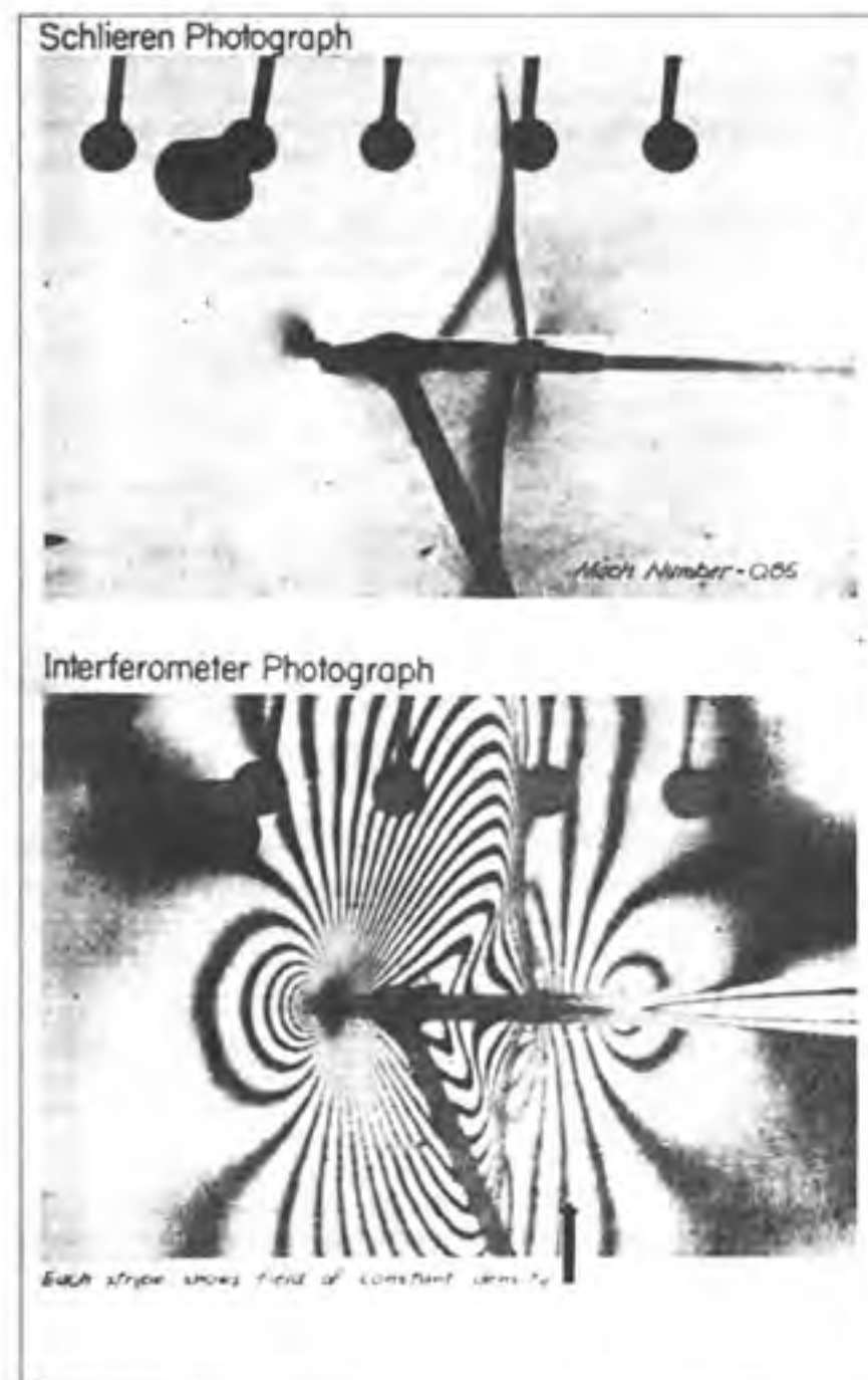
Figure 15—High-Speed Airflow Photographs
