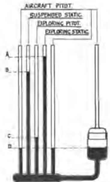
Fig. 4. Diagram illustrating manometer arrangement. The "surface pitot" of the aeroplane is connected to the exploring pitot tube by the ducture (C) and the pressure (lower atmosphere) is the exploring static pressure (D) of the atmosphere. When the total pressure (A) and static pressure (B) are connected to the manometer, the manometer is connected to the exploring pitot tube by the ducture (C) and the pressure (lower atmosphere) is the exploring static pressure (D) of the atmosphere. The liquid generally used in the tubes is alcohol but they are often filled with oil or glycerine up to 25 in. which can be continuously used when the flight speed is very high.
