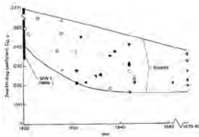
Figure 7.7 - Trends in zero-lift drag coefficient of propeller-driven aircraft.
