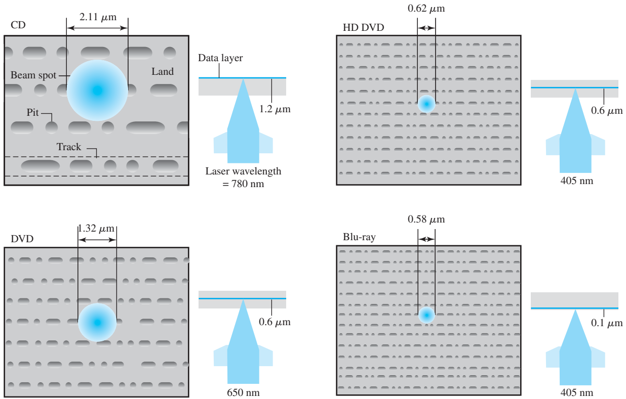
Figure 11.20 Optical Memory Characteristics
