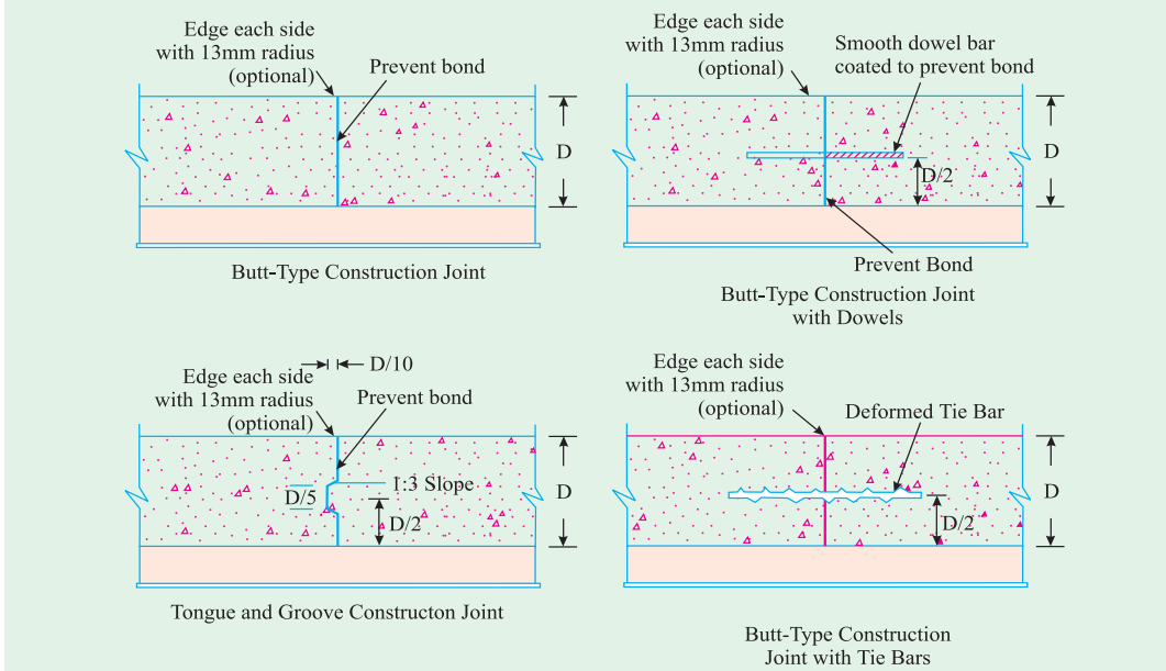
Fig. 9.10. Construction Joints
