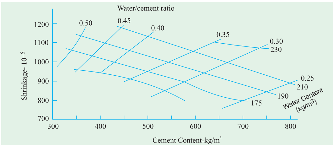
Fig. 9.5. The pattern of shrinkage as a function of cement content, water content, and water/cement ratio; concrete moist-cured for 28 days, thereafter dried for 450 days 9.7
