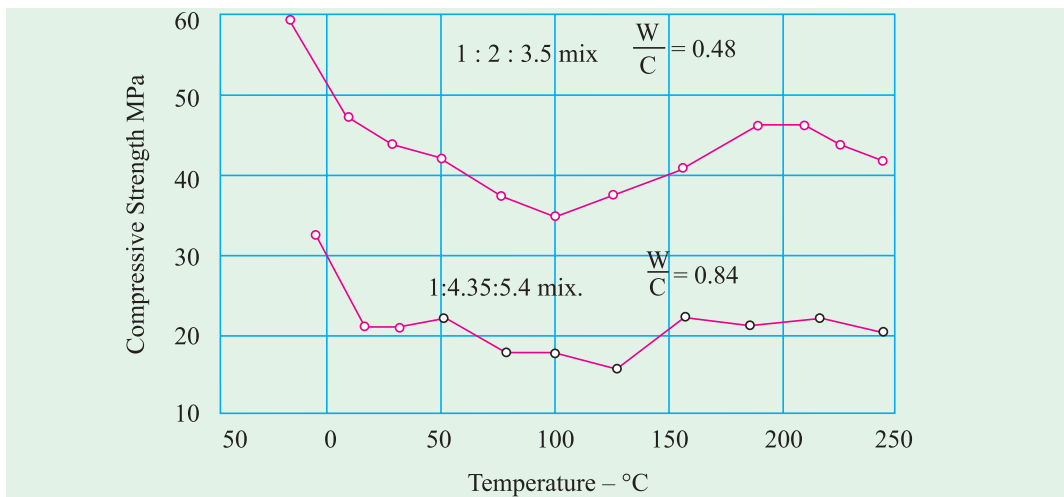
Fig. 9.16. Compressive strength of concrete after heating to different temperatures
