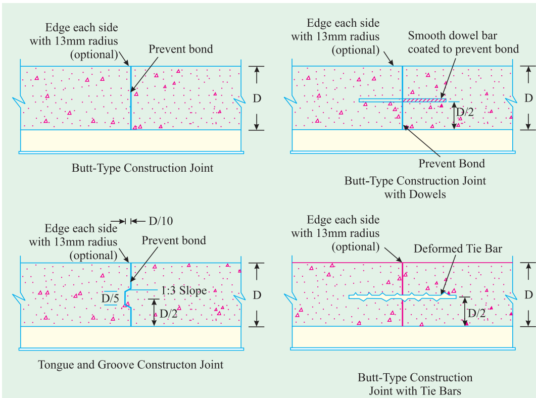
Fig. 9.10. Construction Joints
