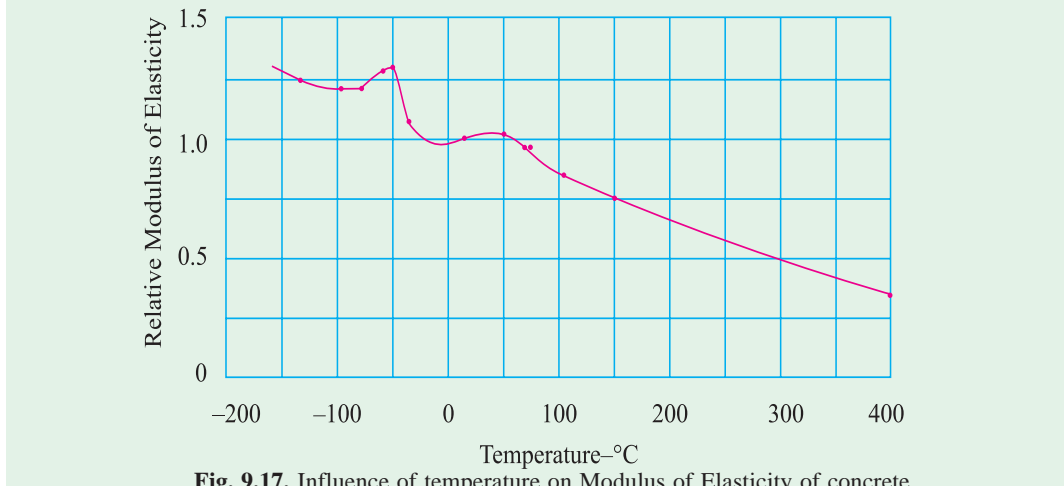
Fig. 9.17. Influence of temperature on Modulus of Elasticity of concrete
