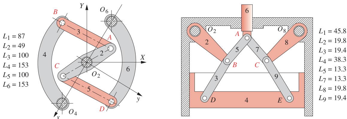
(g) Drum brake mechanism
