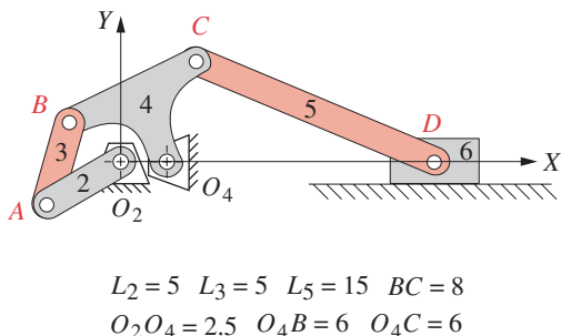
(e) Draglink slider crank
