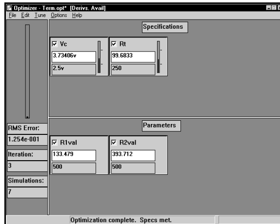
Figure 25 Optimization results for the passive terminator example.
