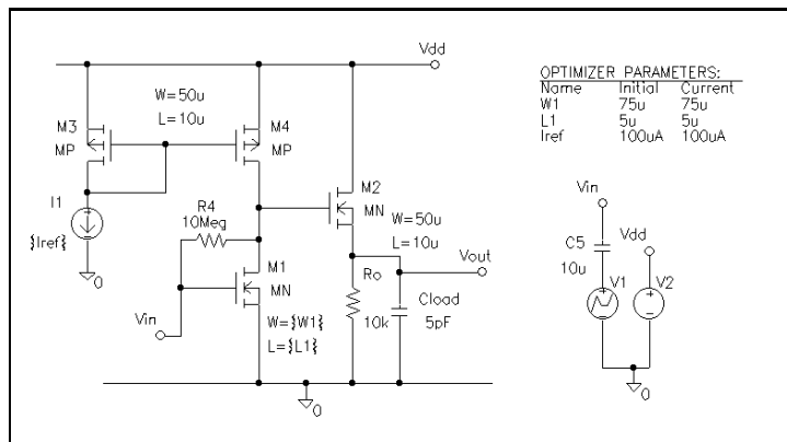
Figure 28 Schematic for CMOS amplifier example, M2.DSN.
