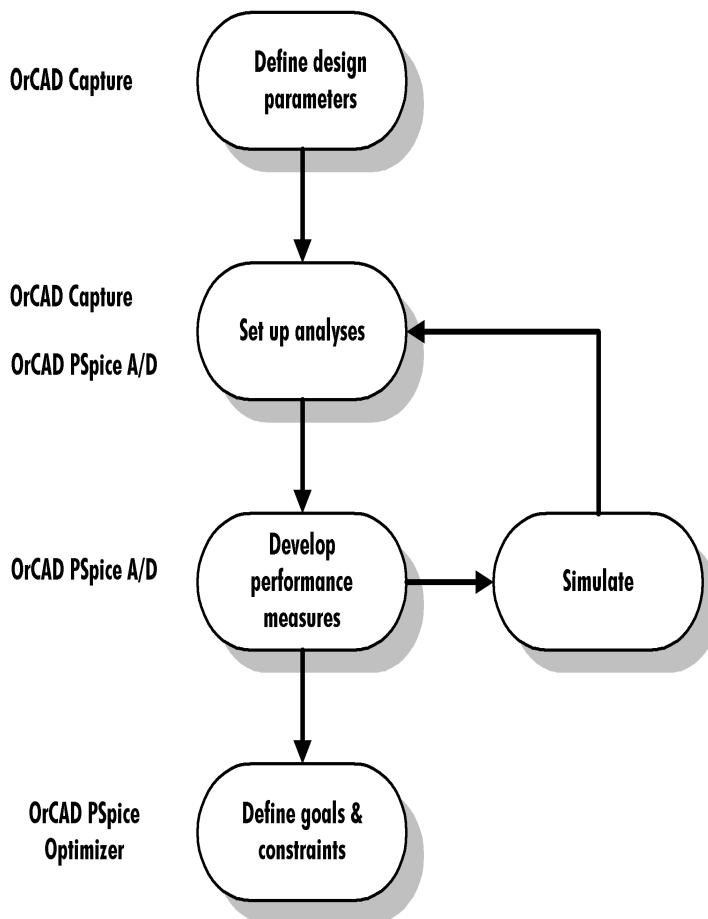
Figure 4 Design flow for setting up the optimization.
