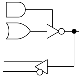
Combinatorial/Active LOW
