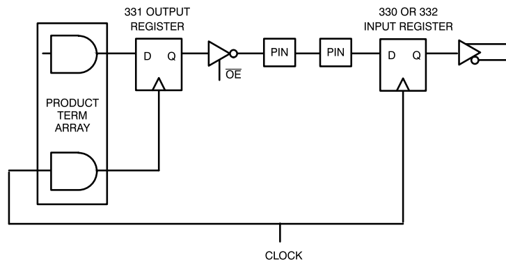
Figure 3. Timing Configurations (continued)
