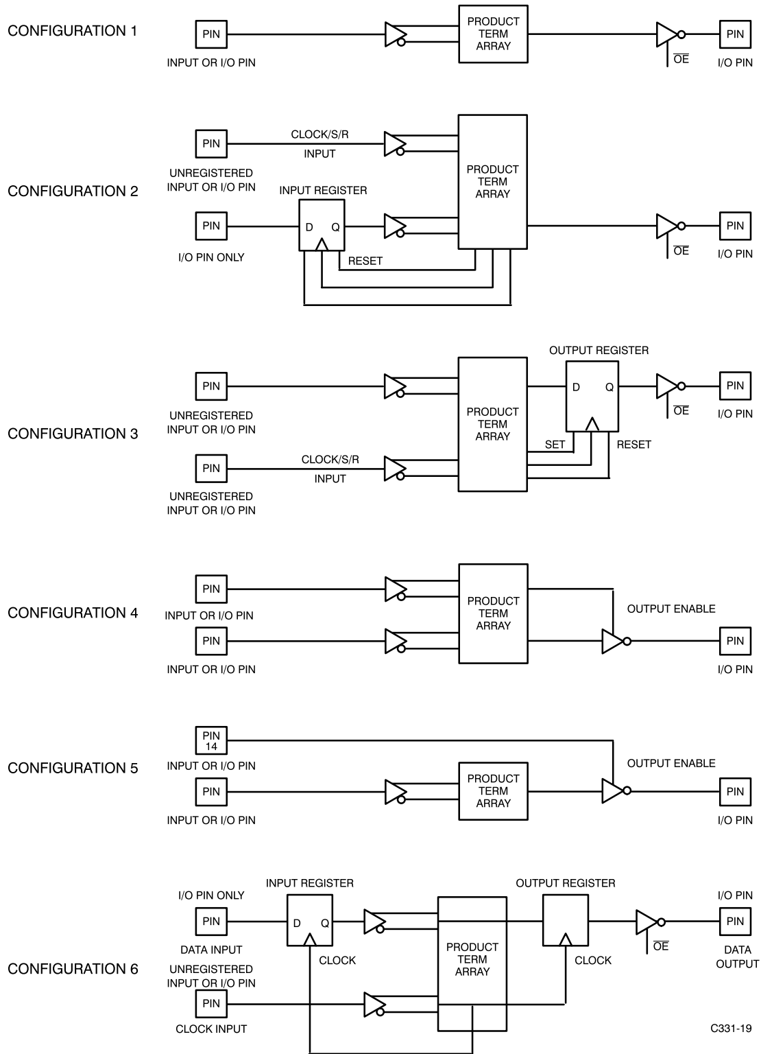
Figure 3. Timing Configurations
