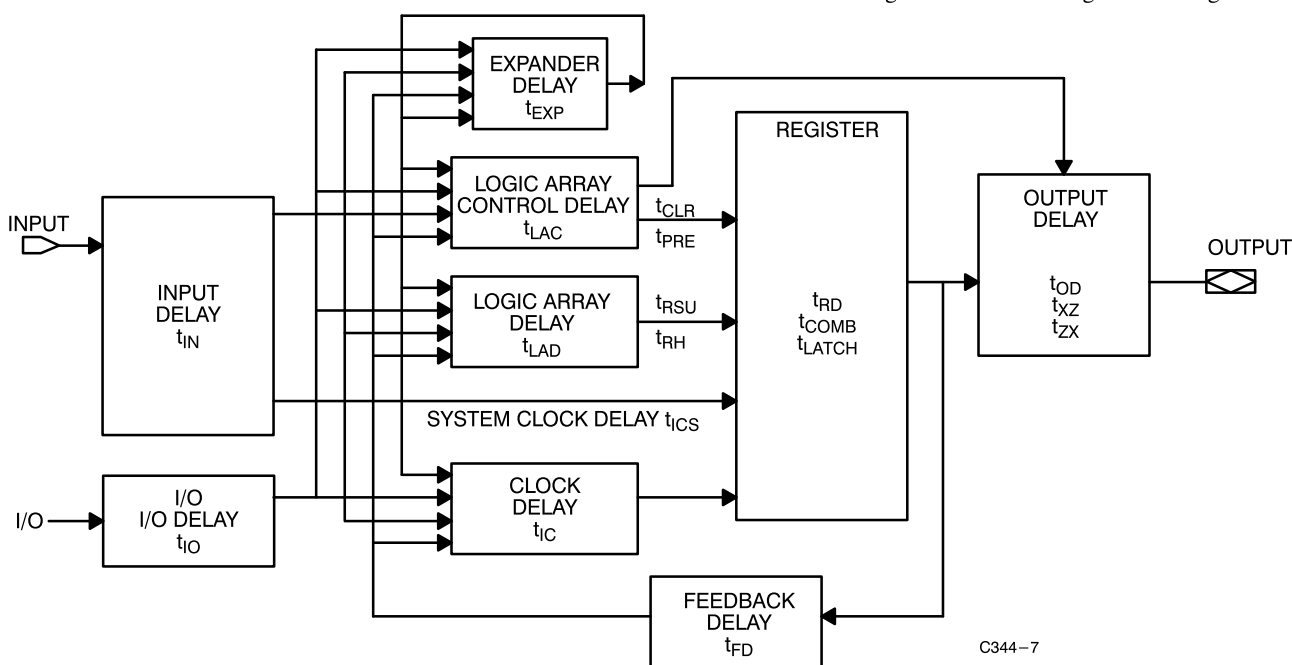
Figure 1. CY7C344/CY7C344B Timing Model
