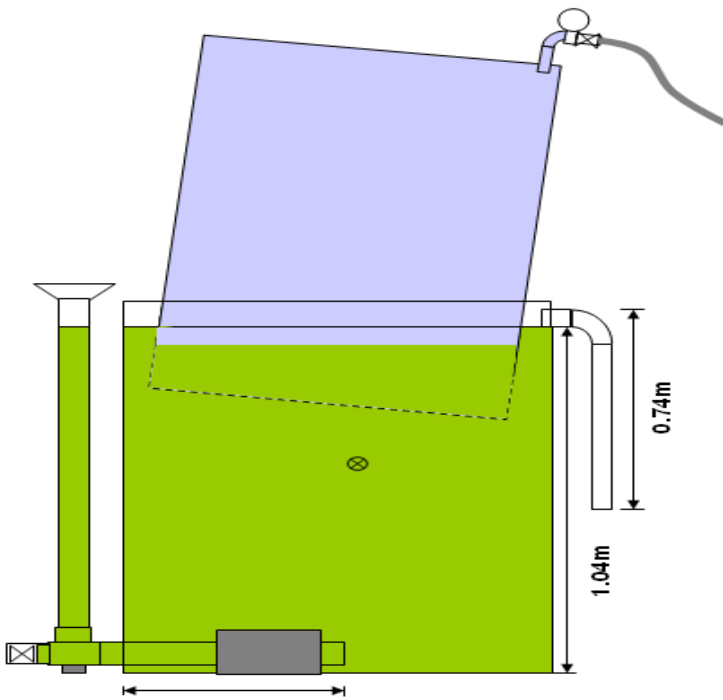
0.51m methane is produced in Gas holder tank
