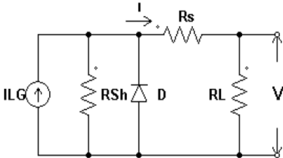
Fig.3 Modified Equivalent circuit of PV cell
