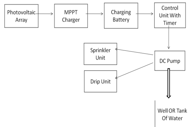
Fig. 8 Block diagram of whole system
