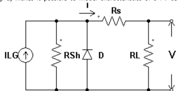
Fig. 2 Equivalent Circuit of a PV Cell
