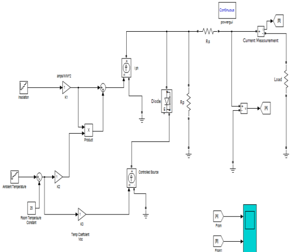
Fig. 5 Simulink model of PV cell (different radiation)
