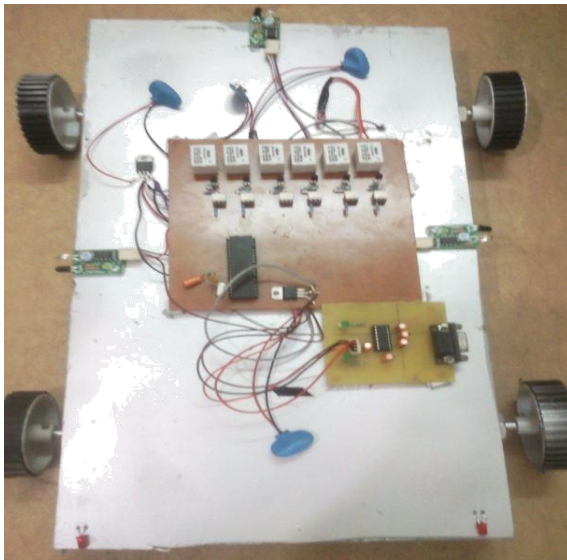
Fig3: Vehicular hardware Module
