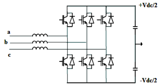
Fig .2 Two level VSC
