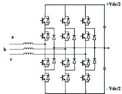
Fig3.Three level VSC
