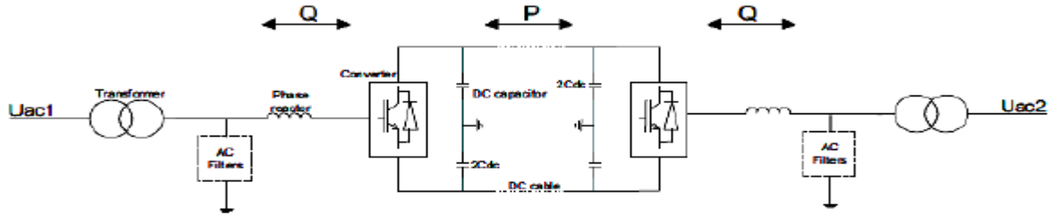
Fig1.Configuration of a VSC-HVDC System
