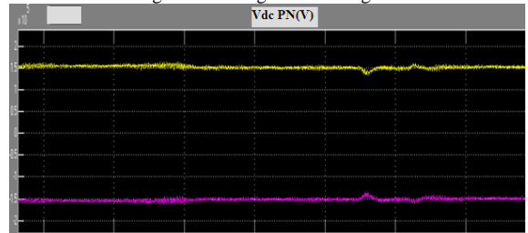
Fig6. DC voltage at sending end
