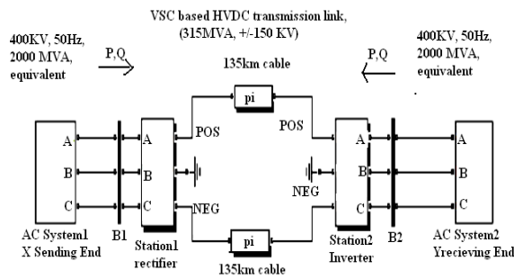
Fig 4 VSC based HVDC transmission link
