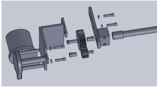
Figure no 6. Overall assembly
