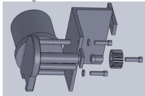
Figure no 4. Motor assembly
