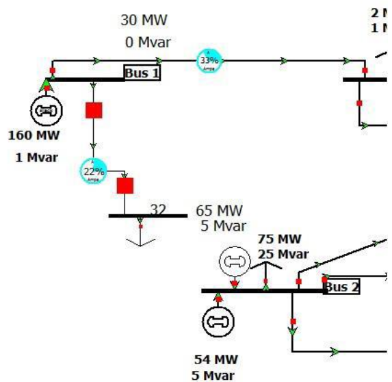
Figure2:- UPFC modelling in Power World Simulator
