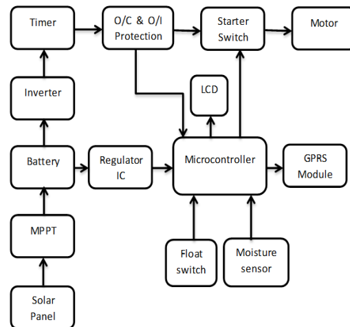
Fig. Block diagram of solar powered smart irrigation system with GPRS
