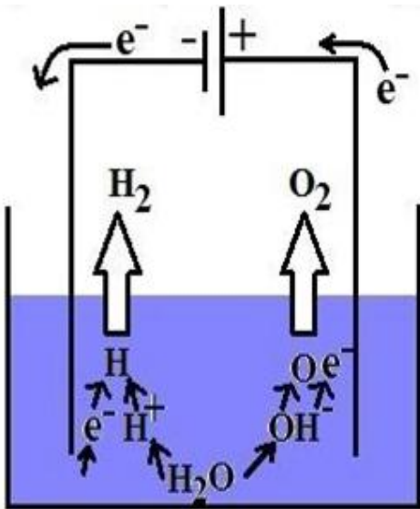
Fig 1 : electrolysis of water
