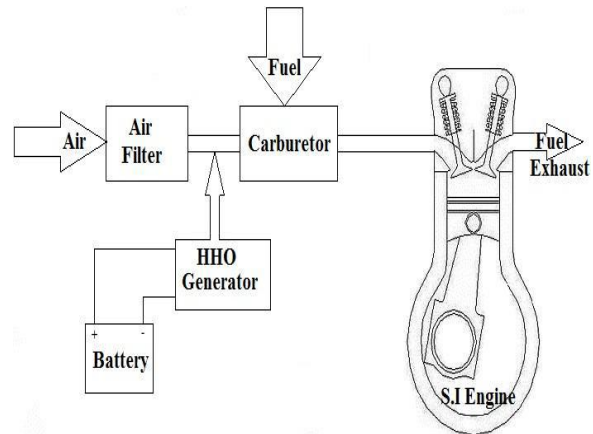
Fig 2 : Schematic illustration of HHO system
